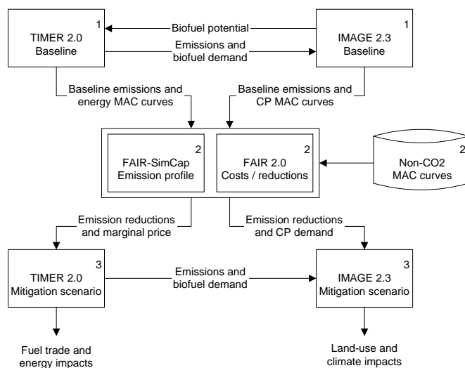
Figure 4.1: Linkage and information flows of the applied modelling framework (note CP = Carbon plantations). Numbers in Figure are explained in the text.
