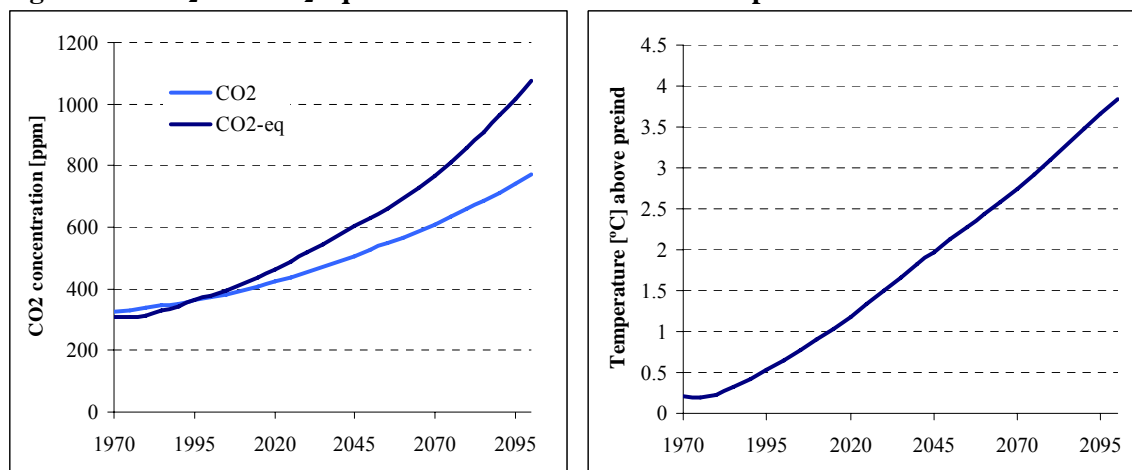
Figure 4.5. CO 2 and CO 2 equivalent concentrations and temperature in the B2 baseline
