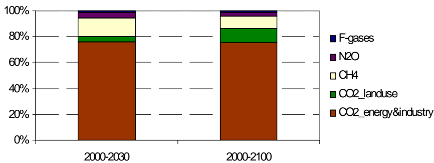
Figure 3.4: Shares by GHG in Cumulative Emissions Reductions in B2-2.6
