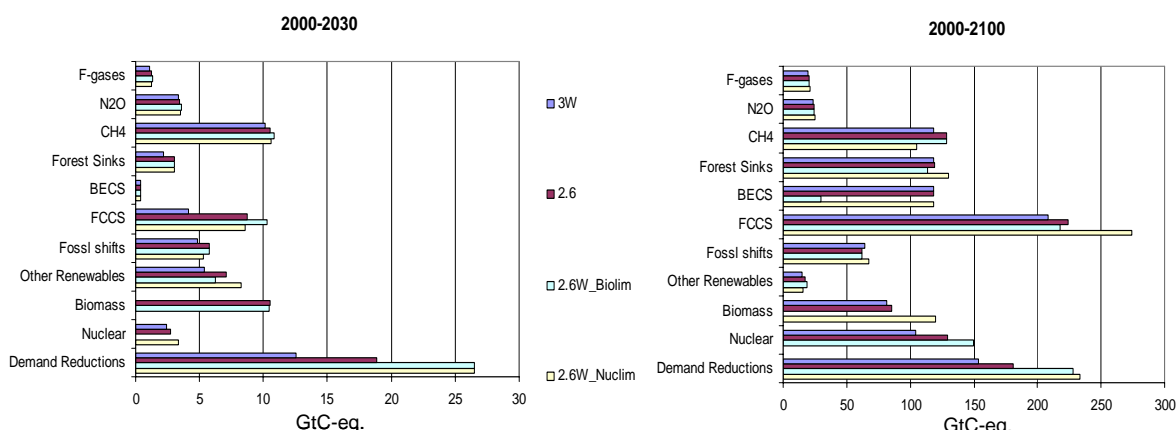
Figure 3.12: Contribution to Mitigation, 2000-2030 and 2000-2100
