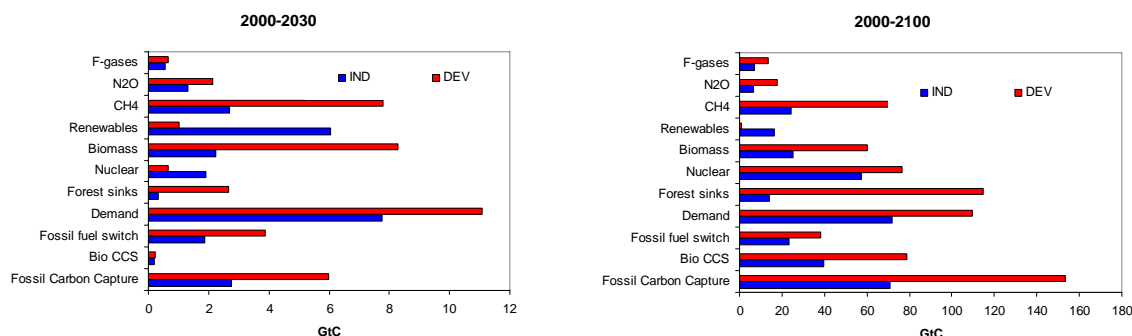
Figure 3.7: Mitigation by Technology, B2_2.6W
