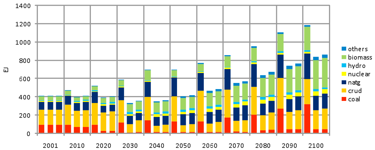
Fig.3-1 Primary energy supply (left: reference, center: 2.6W/m 2 case, and right: 2.9W/m 2 case in each year)
