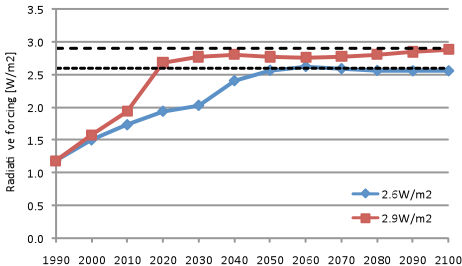
Fig. 2-1 Pathways of radiative forcing (AIM/Impact [Policy])
