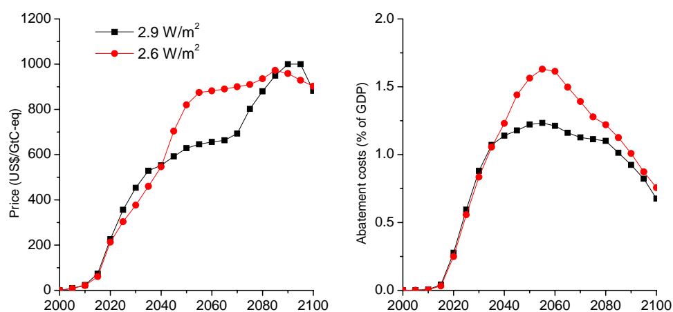
Figure 4.12: Carbon price and abatement costs of the 2.6 and 2.9 scenario
