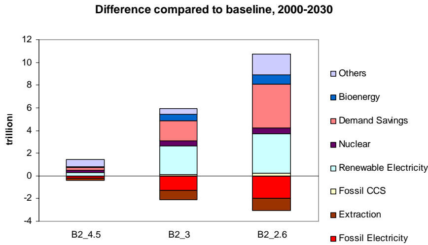
Figure 3.10: Additional Investments for Climate Mitigation
