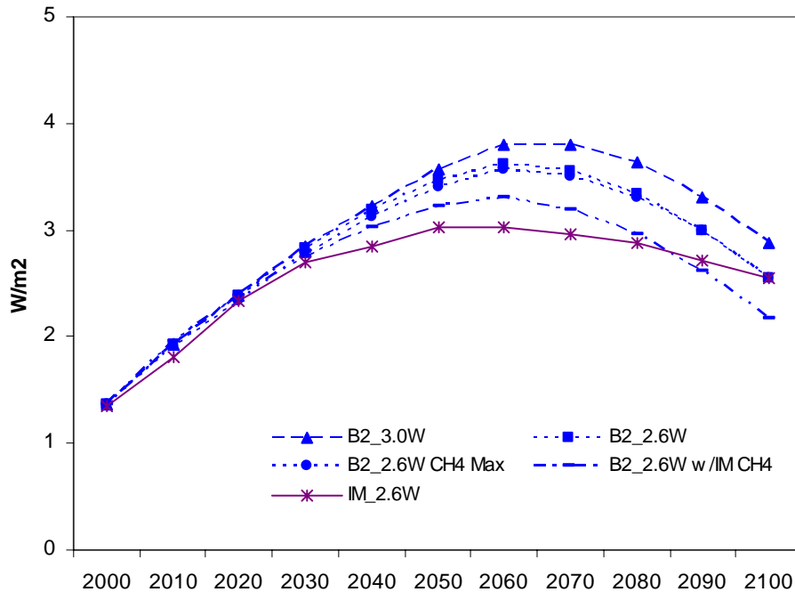
Figure 3.14: Overshoot in Radiative Forcing
