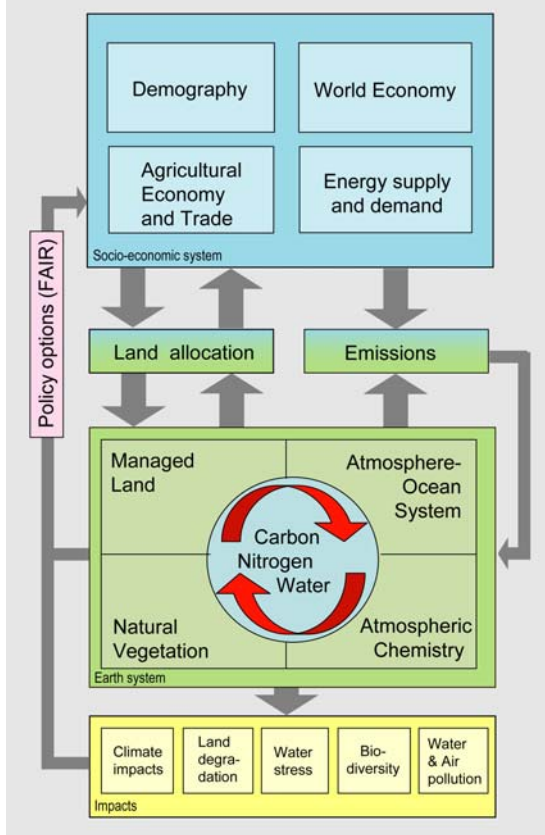
Figure A1: IMAGE 2 Integrated Assessment Framework.
