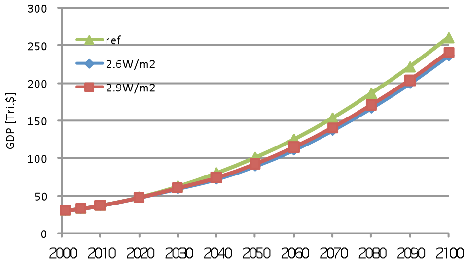
Fig.3-4 GDP
