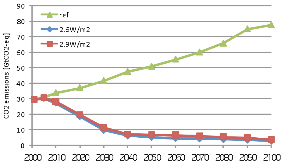
Fig.3-2 Global CO 2 emissions
