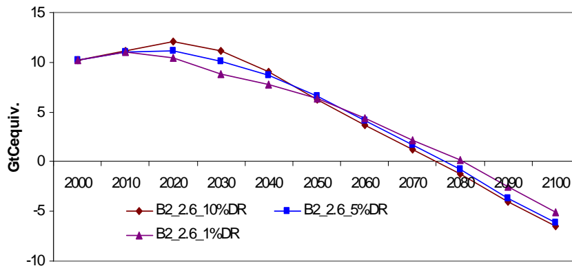
Figure 3.3: Implications of Alternative Discount Rates
