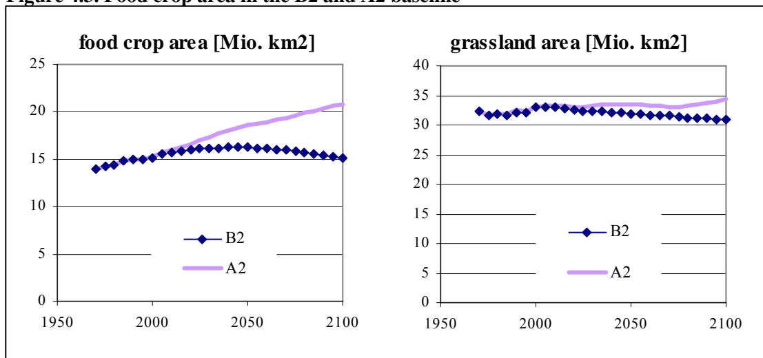
Figure 4.3. Food crop area in the B2 and A2 baseline
