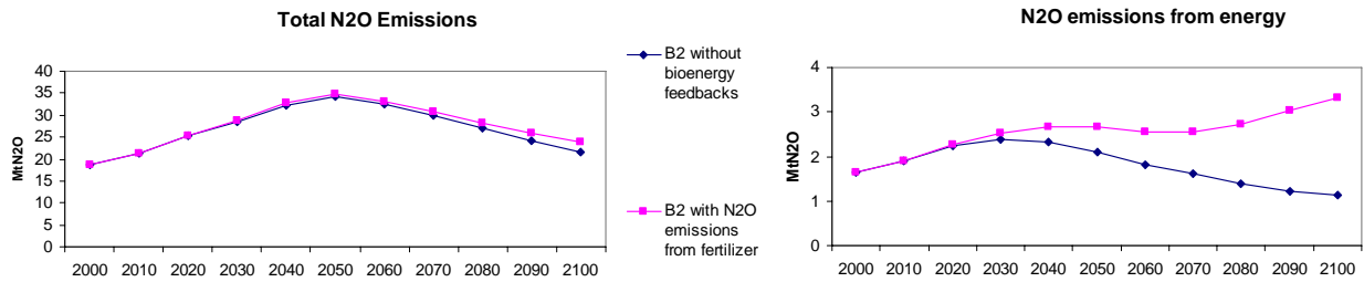
Figure 3.1: Increase in N 2 O emissions due to bioenergy feedbacks
