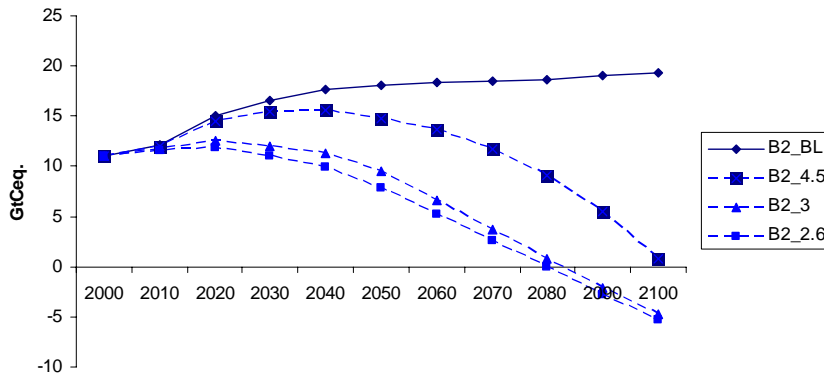
Figure 3.2: GHG Emissions
