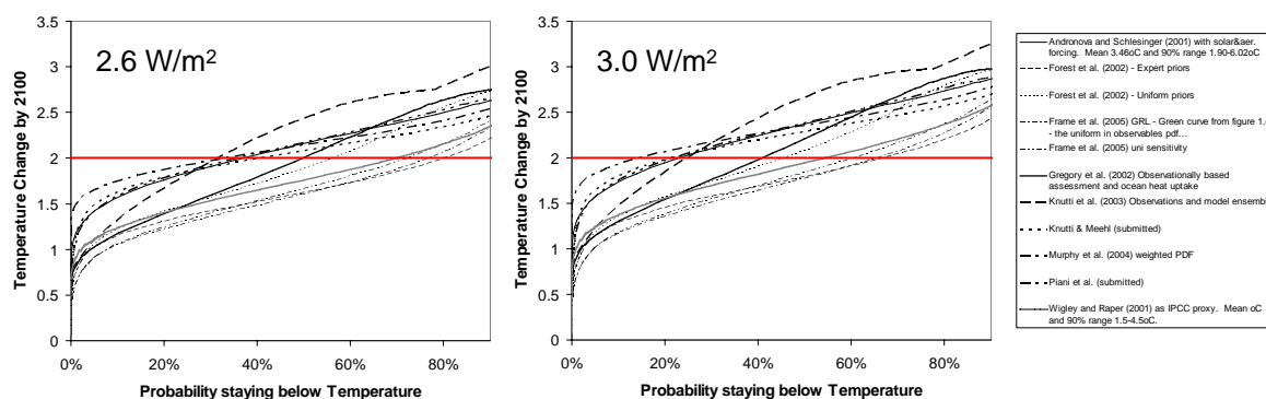
Figure 3.16: Probabilities of staying below specific temperature thresholds (B2-2.6 left-hand panel; and B2-3 right-hand panel) *
