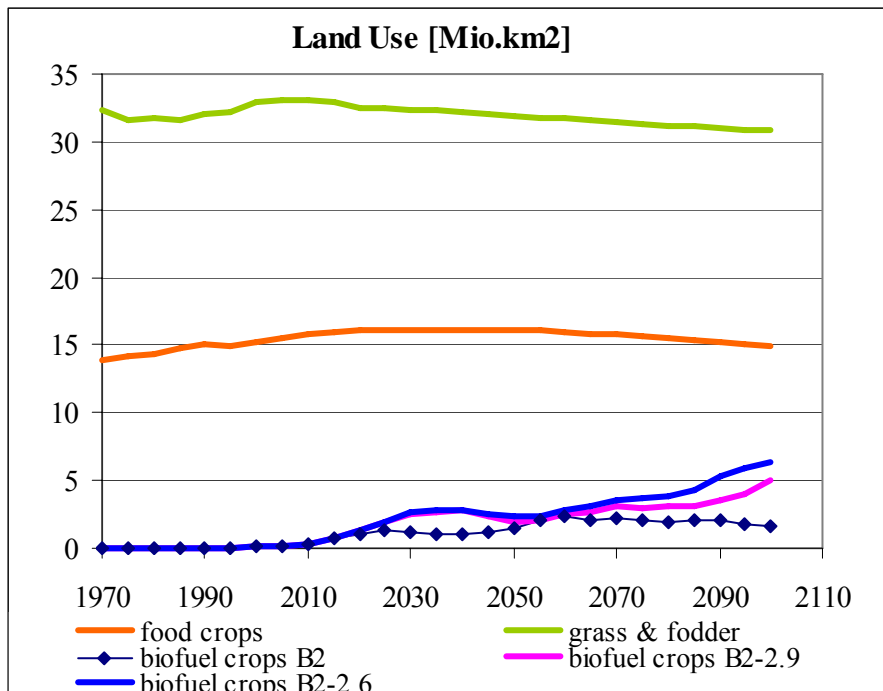
Figure 4.10: Land use in the B2 baseline, the B2-2.9 and B2-2.6 scenario.
