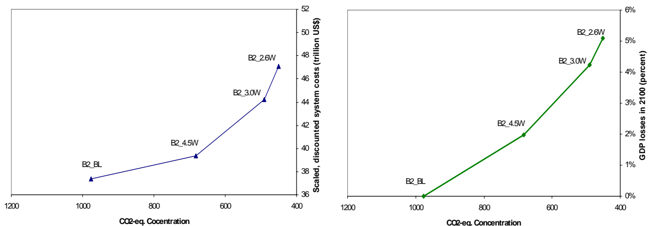
Figure 3.9: Costs of Climate Mitigation in 2100
