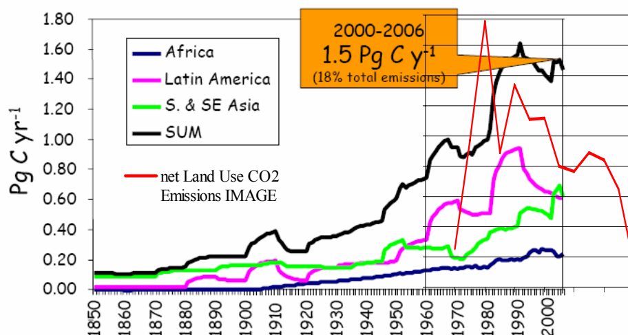
Figure 4.16. IMAGE land use CO 2 emissions compared to Houghton (unpublished) and Canadell et al. PNAS (as shown in an ESSP presentation).
