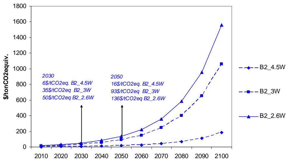
Figure 3.11: GHG Shadow Prices , $/ton CO 2 equiv. (2000 US$)
