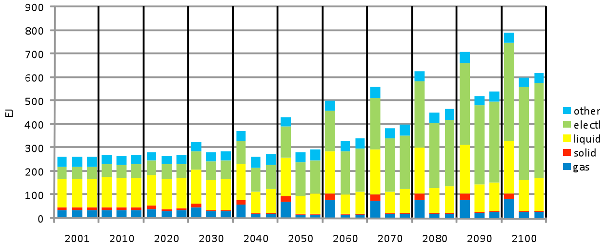
Fig.3-3 Final energy (reference, 2.6W/m 2 case, and 2.9W/m 2 case in each year)
