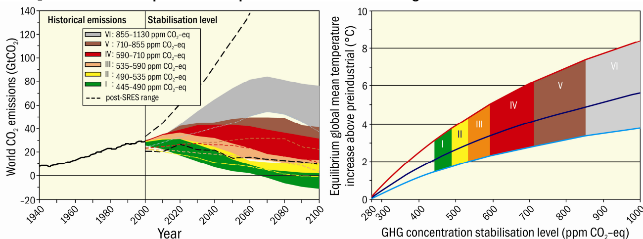
23 Figure SPM.8. Global CO 2 emissions for 1940 to 2000 and emissions ranges for groups of stabilisation 24 scenarios from 2000 to 2100 (left-hand panel); and the corresponding relationship between the stabilisation target 25
