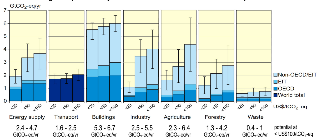
Figure SPM.7. Estimated economic mitigation potential by sector in 2030 from bottom-up studies, compared to the respective baselines assumed in the sector assessments. The potentials do not include non-technical options such as lifestyle changes. {Figure 4.1} Notes:
