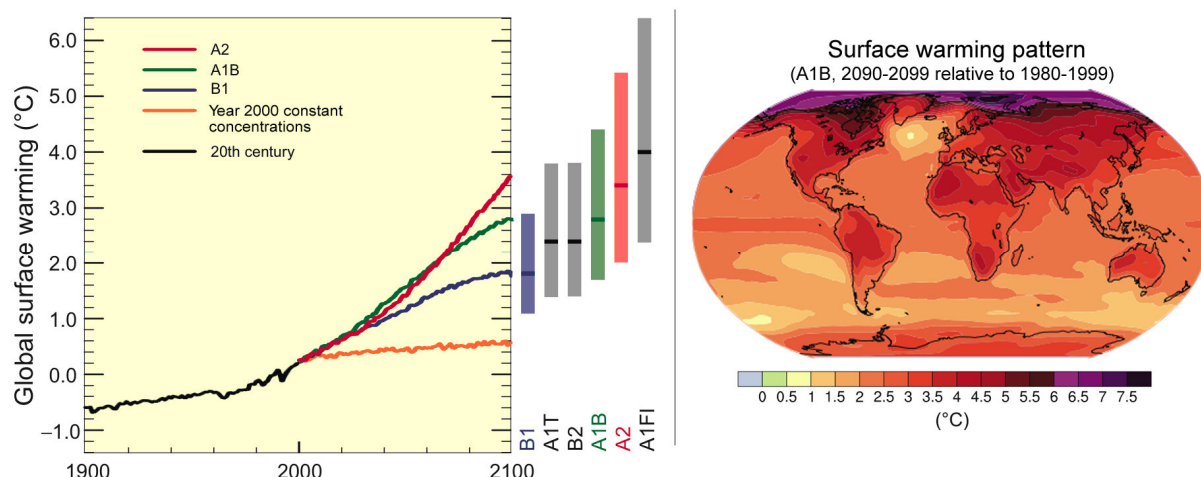
2 3 Figure SPM.5. Left panel: Solid lines are multi-model global averages of surface warming for the SRES 4 scenarios A2, A1B and B1, shown as continuations of the 20 th century simulations. The orange line is for an 5 experiment where concentrations were held constant at year 2000 values. The bars in middle of figure indicate 6 the best estimate (solid line within each bar) and the likely range assessed for the six SRES marker scenarios at 7 2090-2999. Right panel: Projected surface temperature changes for the late 21 st century (2090-2099). The map 8 shows the multi-AOGCM average projection for the A1B SRES scenario. All temperatures are relative to the 9 period 1980-1999. {Figure 3.2}
